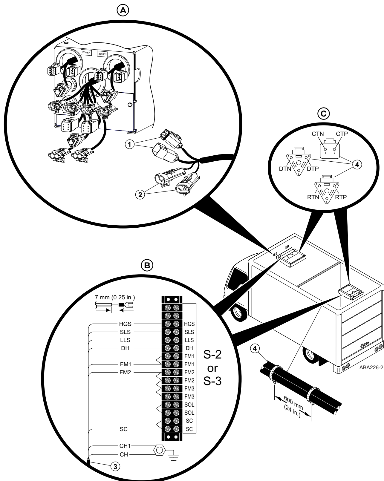
Figure 47. Wire Connections to S-2 or S-3 Evaporators
