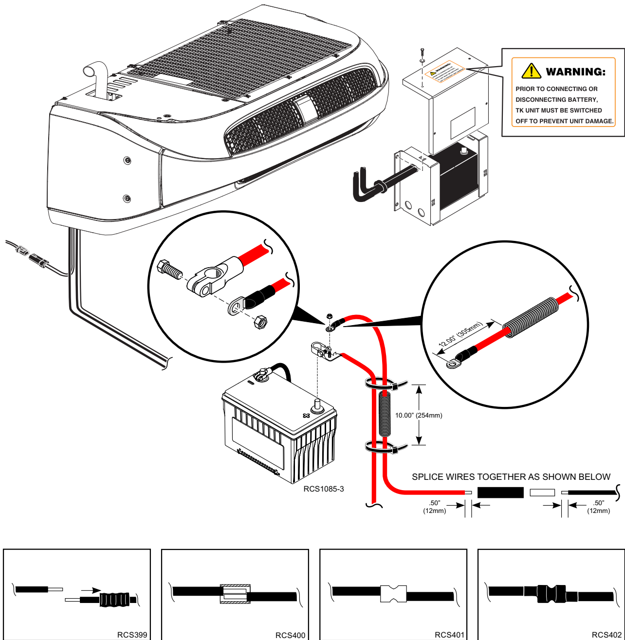
Figure 51. Battery and Fuel Pump Connections Shown
