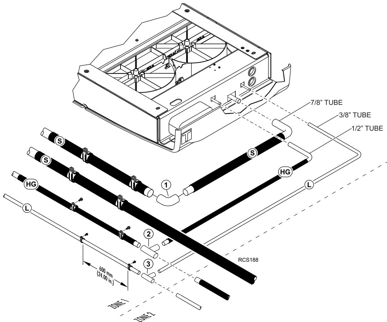
Figure 42. Evaporator Connections
