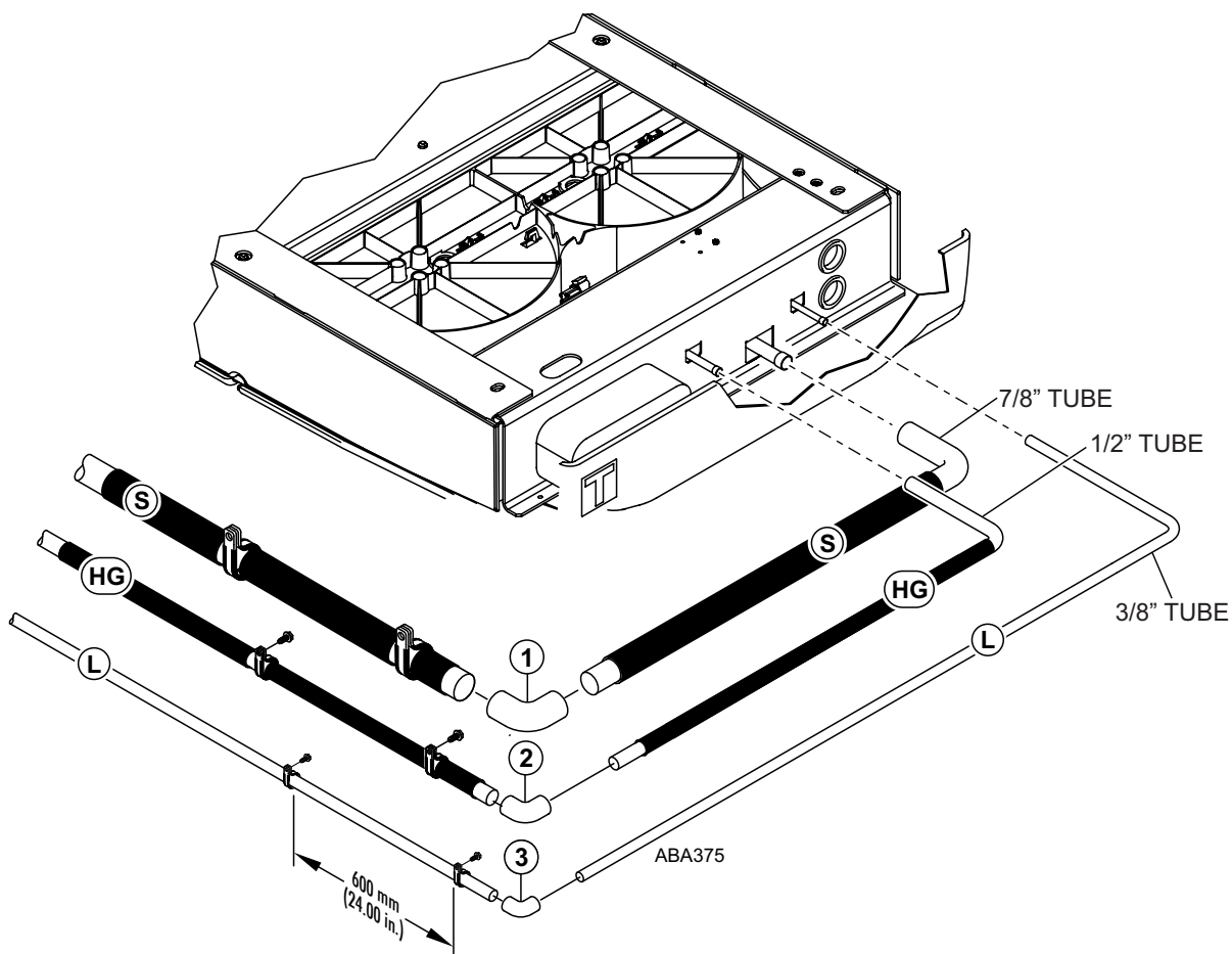
Figure 46. Evaporator Connections
