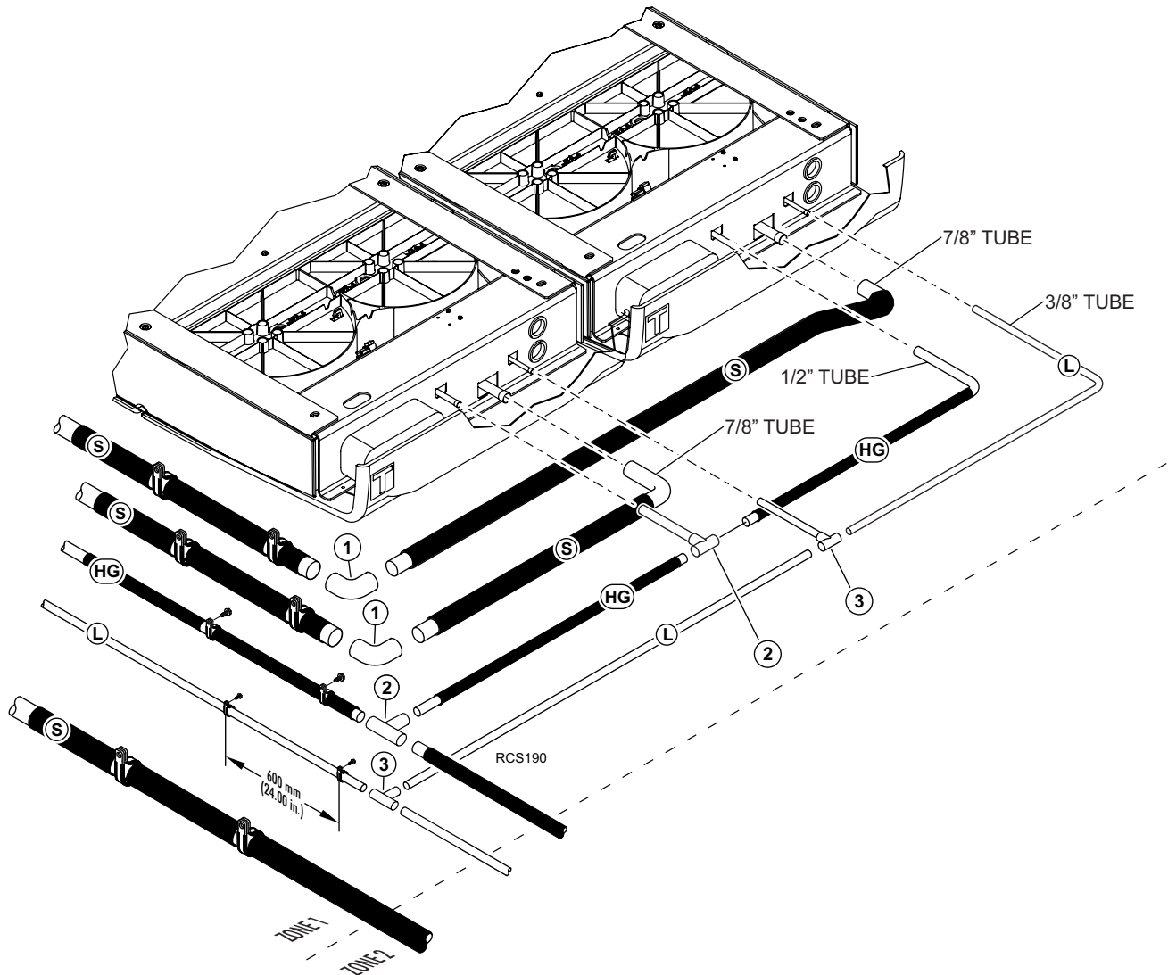
Figure 44. Evaporator Connections Shown
