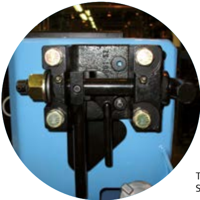
Thermo King patented SGCO Dual-Clamp Mount
