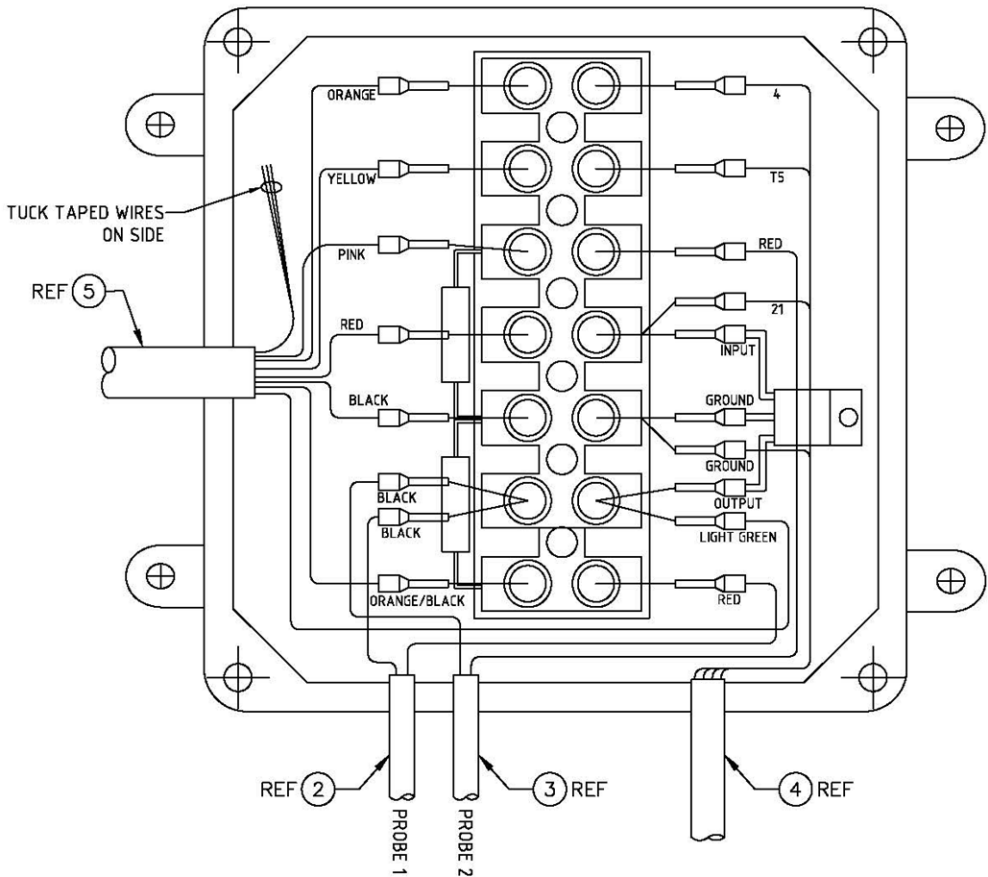
SECTION 6.8 ST9100 JUNCTION BOX
