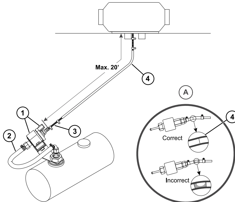
Figure 29. Tank Mounted Fuel Pump Shown.
