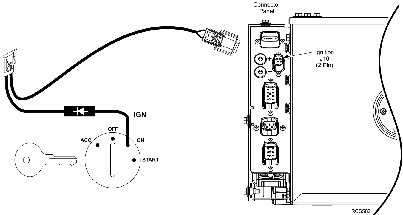
Figure 23. Ignition Switch Harness Connections Shown.
