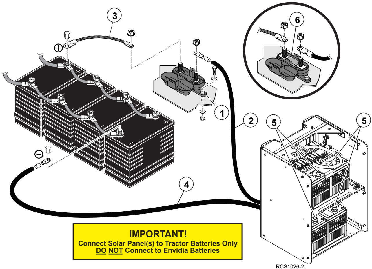
Figure 35. Battery Cables and Fuse Installation.
