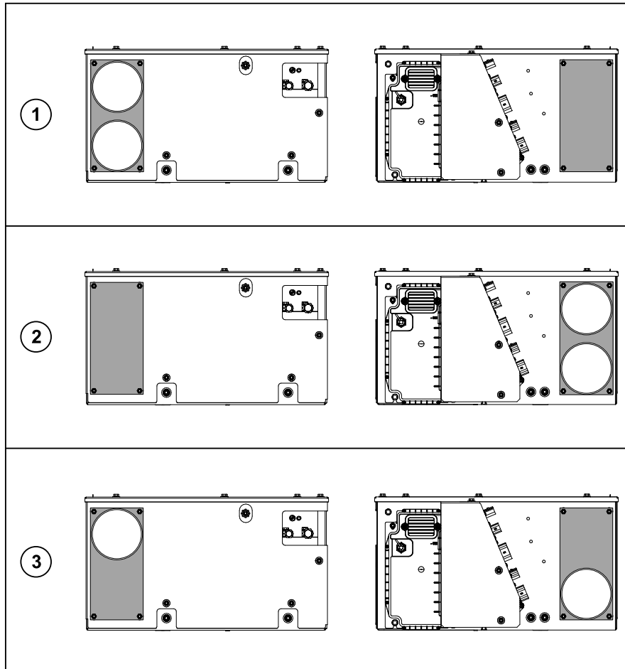
Figure 16. Discharge Air Outlets shown.
