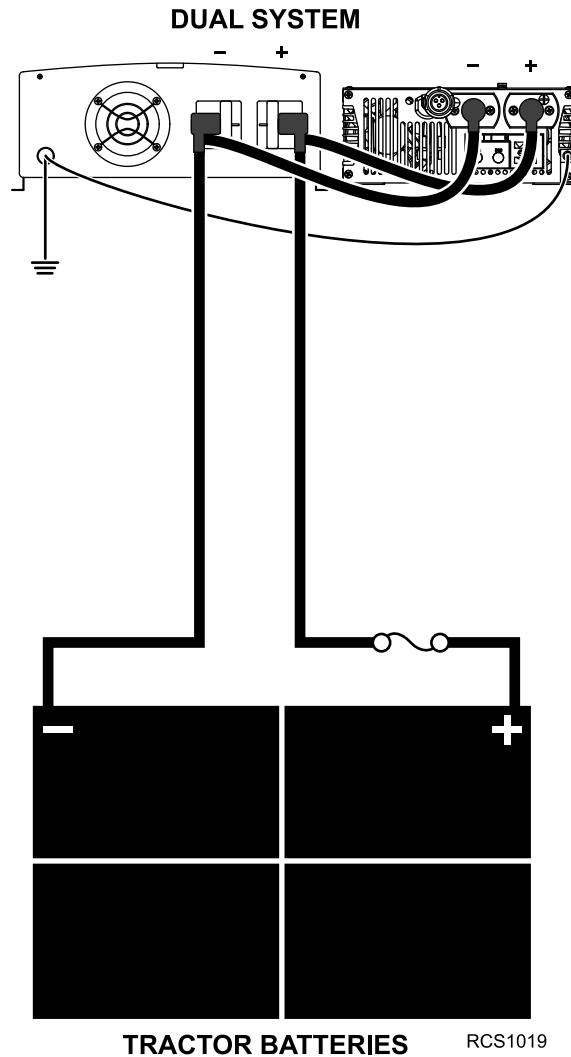
Figure 34. Dual System Connections to Battery Shown.
