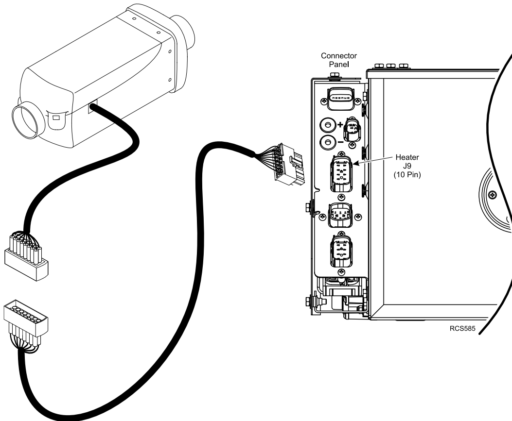
Figure 26. Heater Harness to Evaporator/Control Box Connection Shown.
