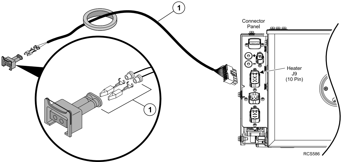
Figure 31. Heater Fuel Pump Connections Shown.
