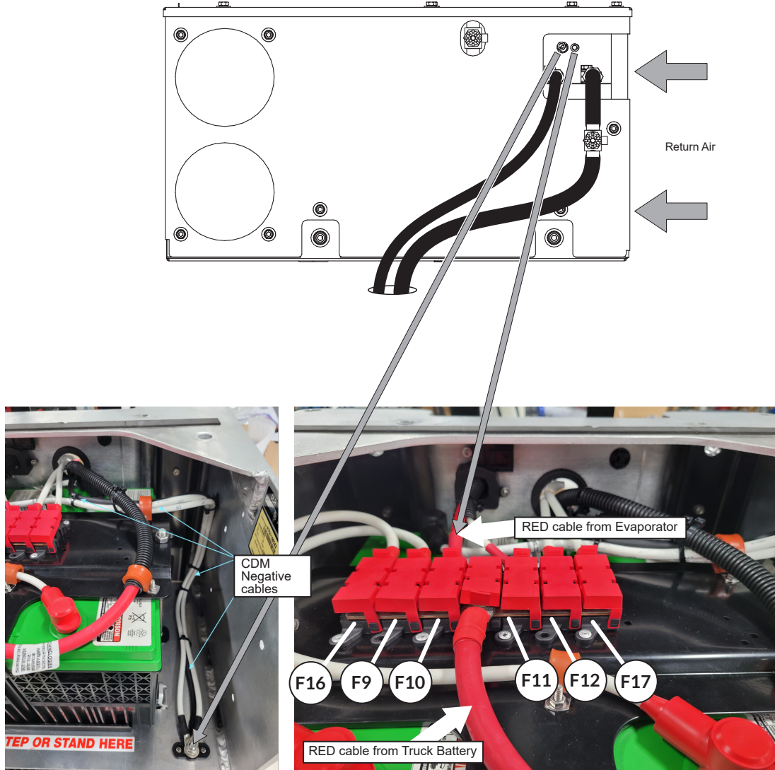
Figure 20. Cable connections shown.
