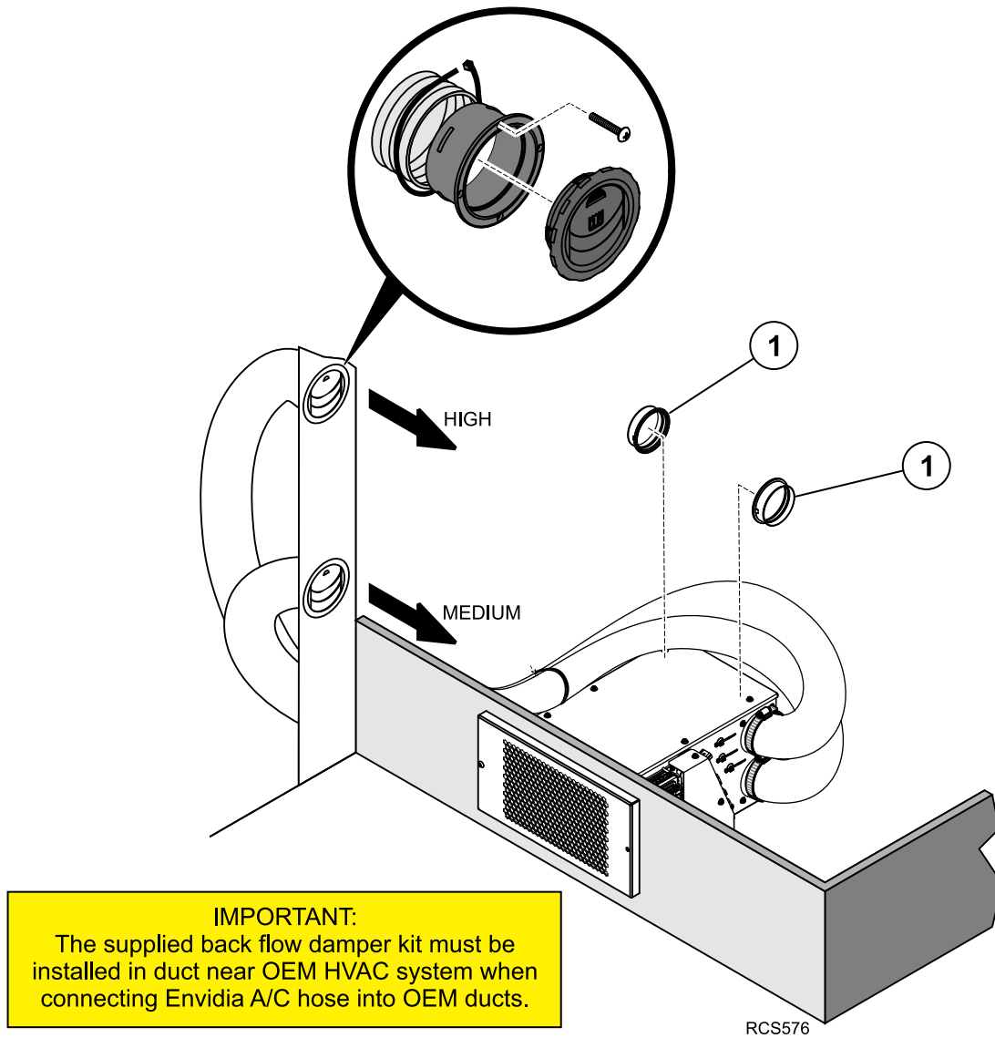
Figure 17. Typical A/C Duct locations shown.
