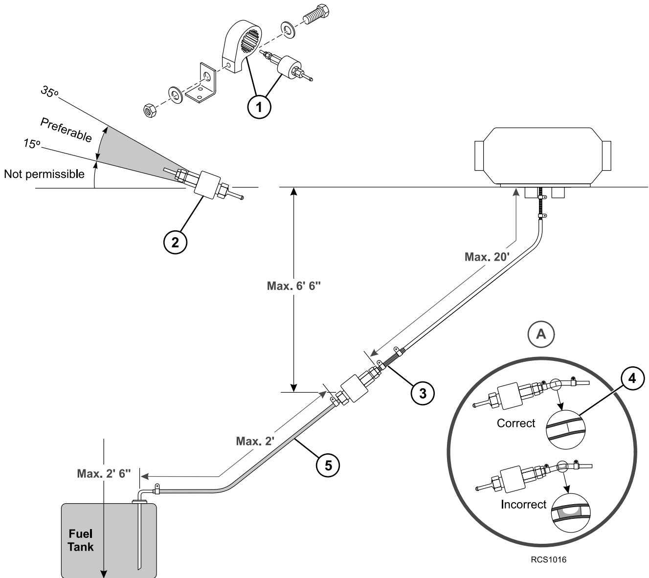
Figure 30. Remote Mounted Fuel Pump with L-Bracket Shown.
