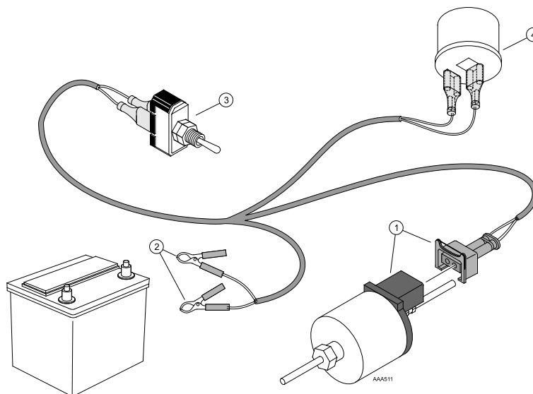
Figure 36. Heater Fuel Pump Priming Harness Connections.
