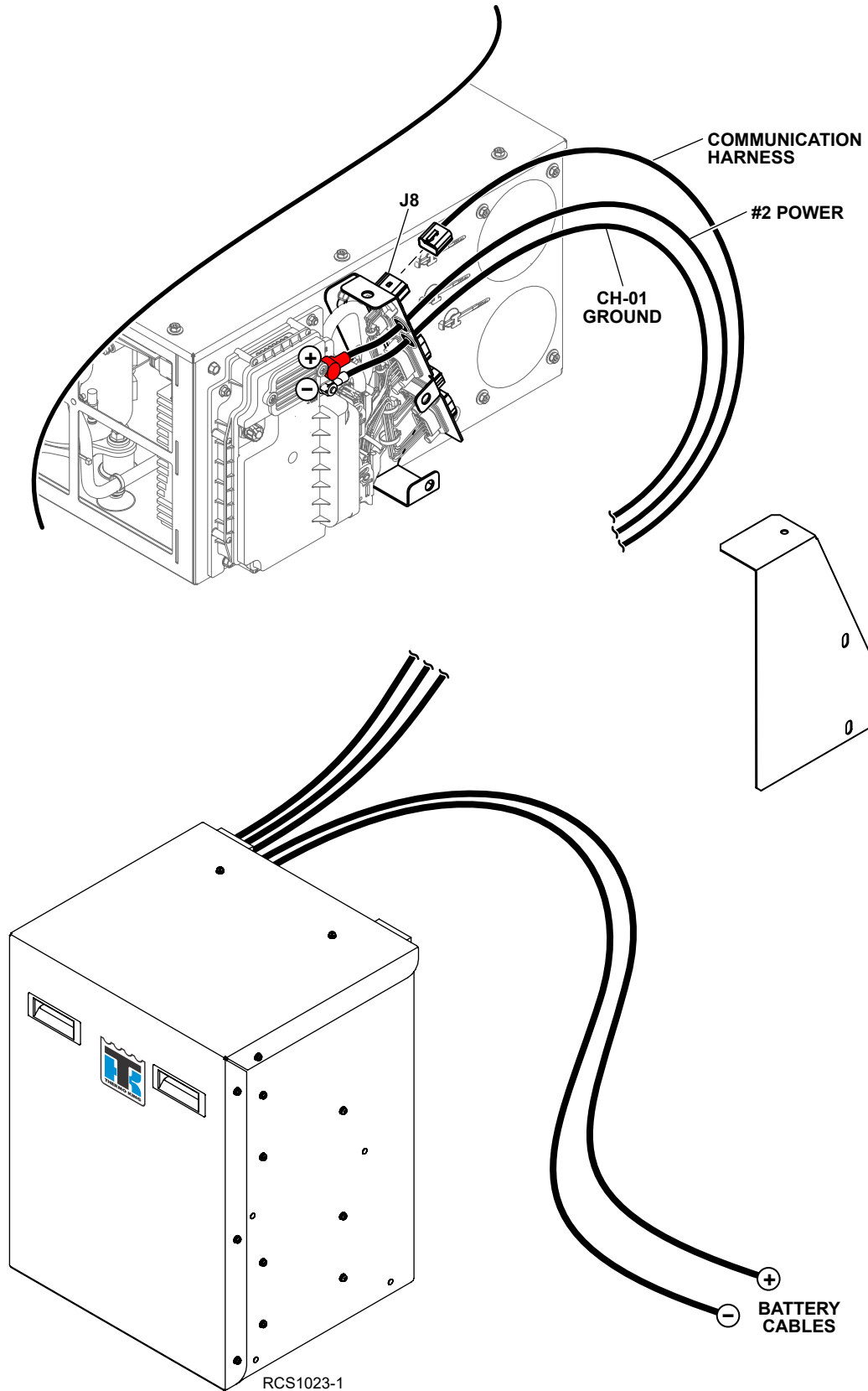
Figure 19. Cable Connections Shown.
