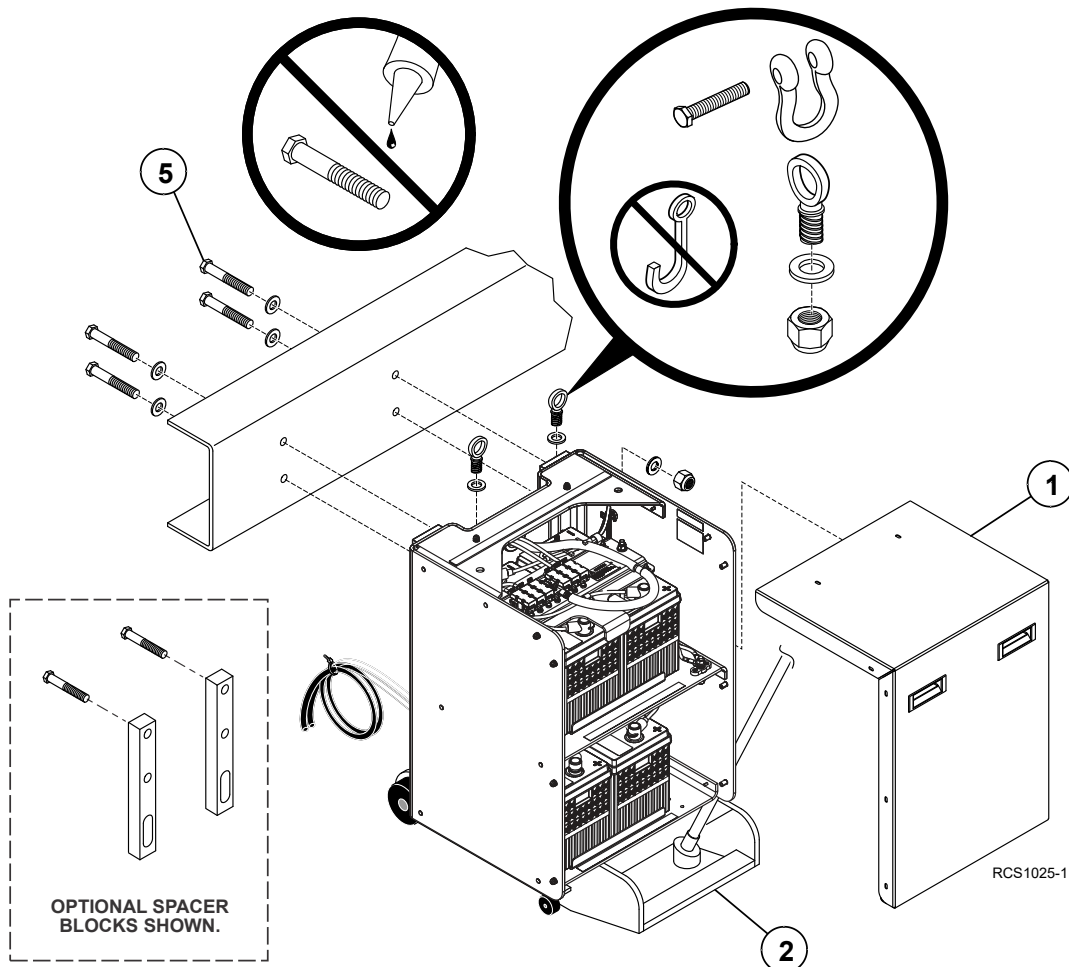
Figure 3. Optional Installation Method – Direct Mount.
