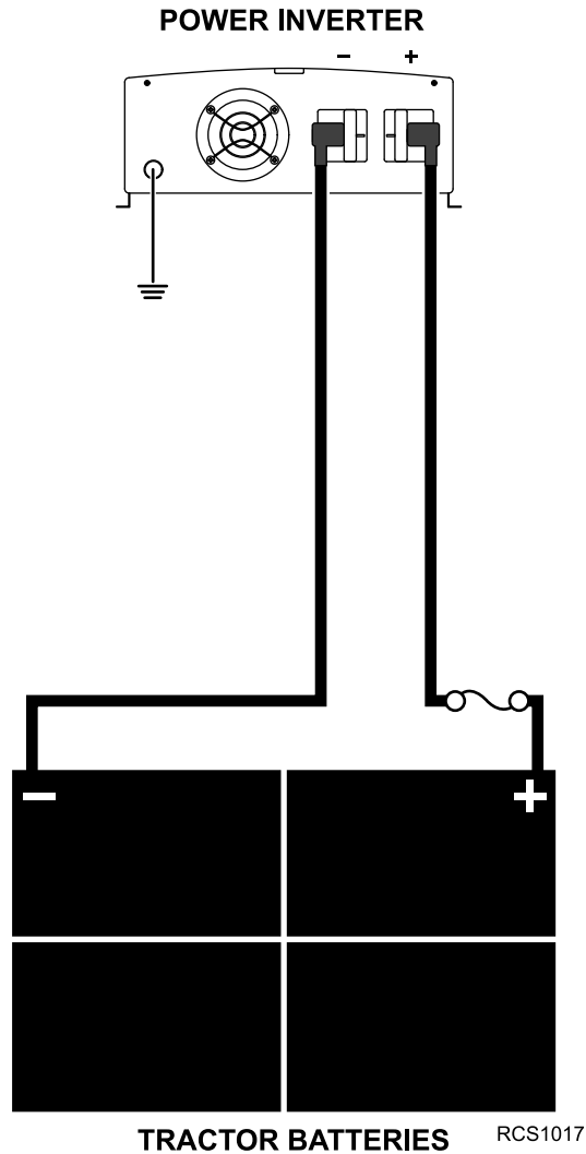
Figure 32. DC/AC Power Inverter Connections to Battery Shown.
