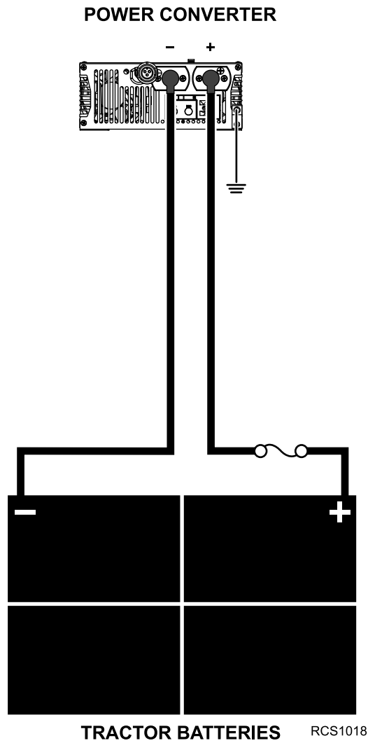
Figure 33. AC/DC Shore Power Connections to Battery Shown.
