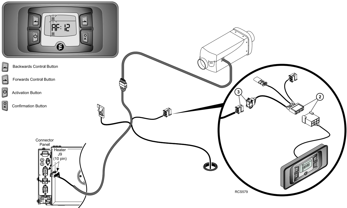
Figure 37. Heater Diagnostic Connections Shown.
