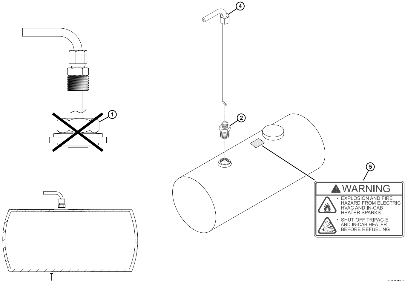
Figure 27. Direct Tank Installation – with OEM Fuel Tank Fittings.
