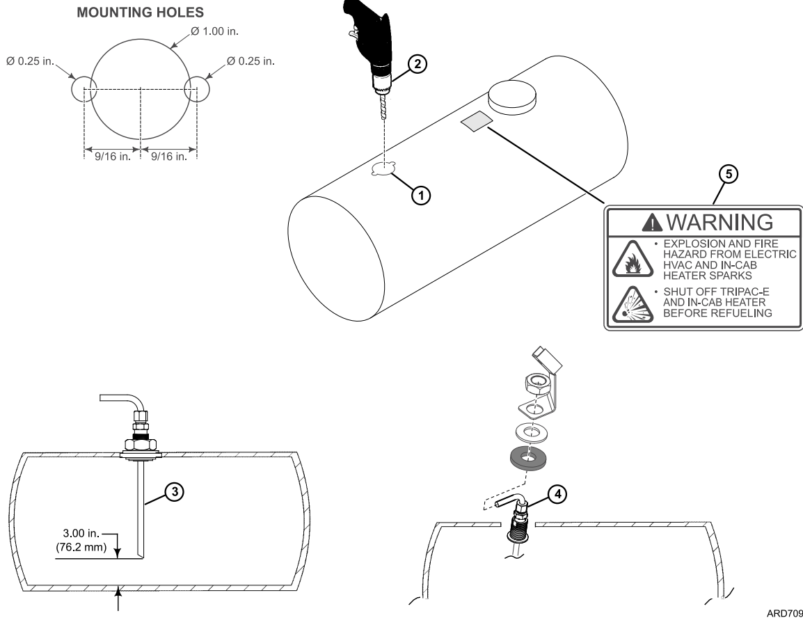
Figure 28. Fuel Pickup Tube Installation – Drilling Hole in Tank.
