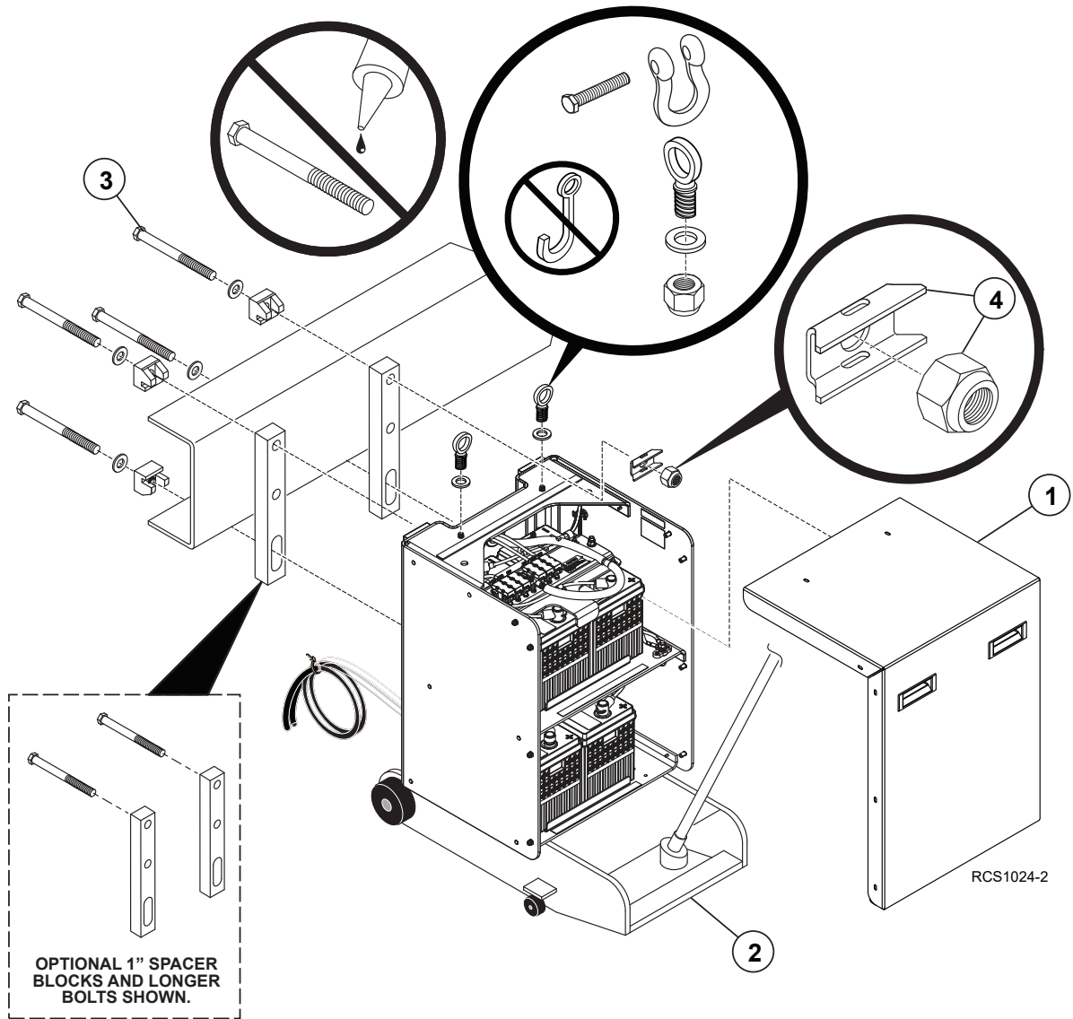
Figure 2. Standard Installation Method – Mounting Claws
