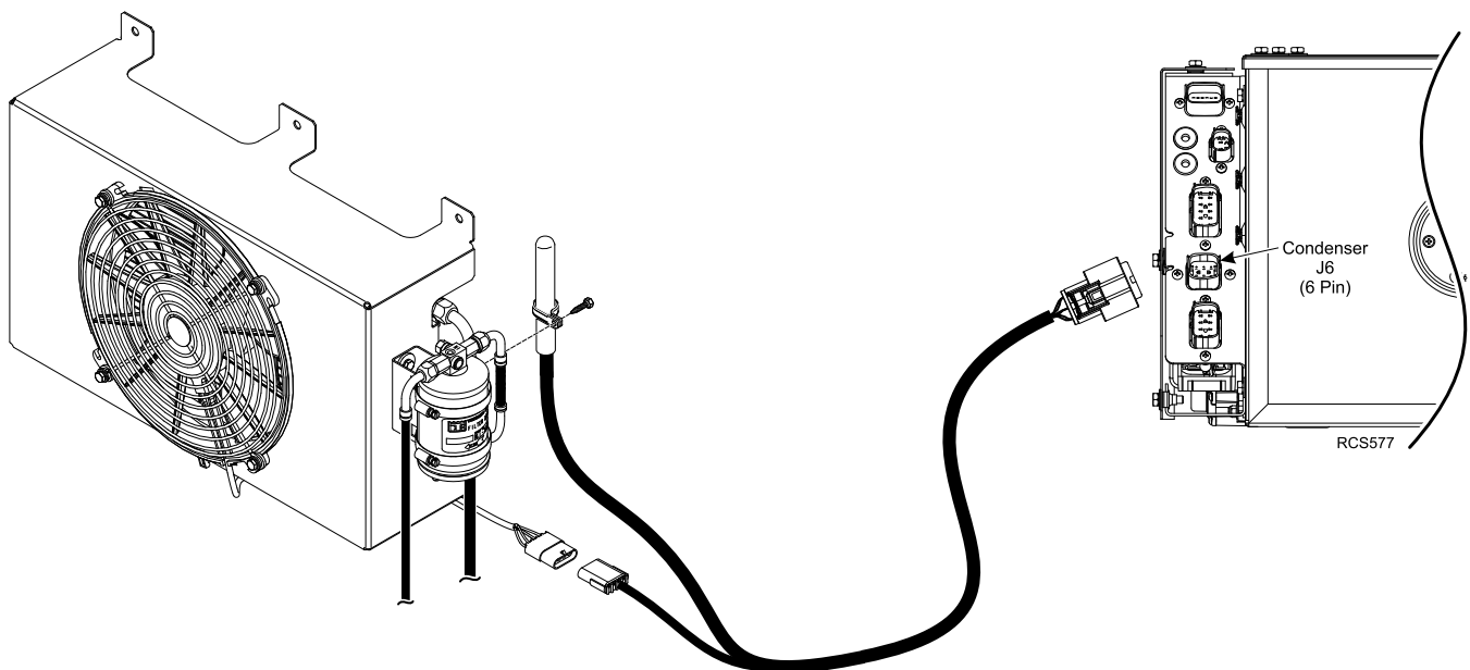
Figure 22. Condenser Harness and Sensor Harness Connections Shown.
