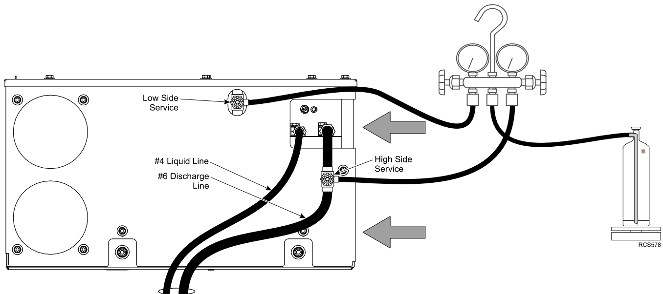
Figure 38. TriPac Envidia Shown Connected to Refrigerant Bottle.
