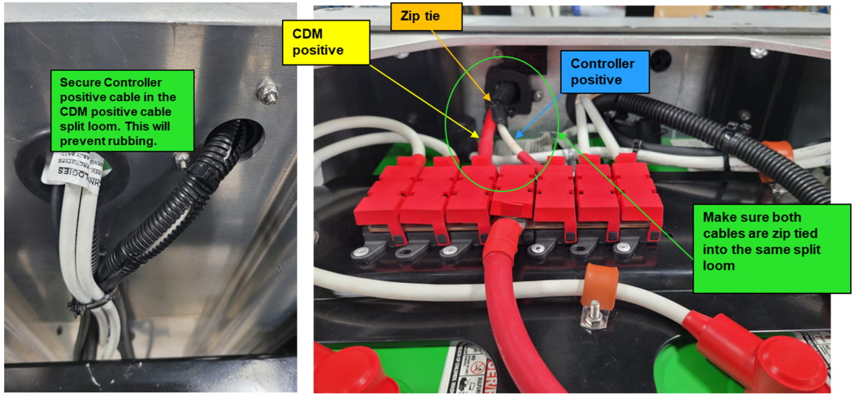
Figure 21. Evaporator/Control Box to Battery Box Connections shown.
